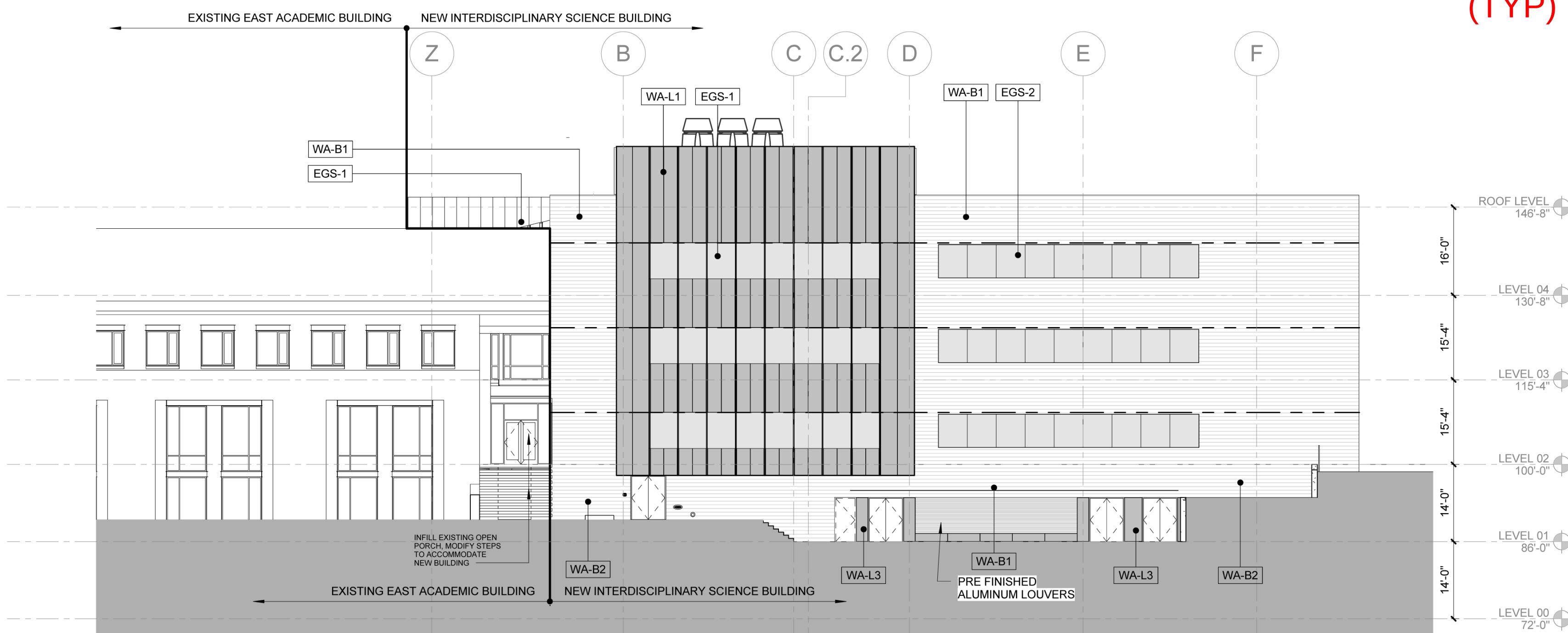
2 EXTERIOR EAST 1/16" = 1'-0"
