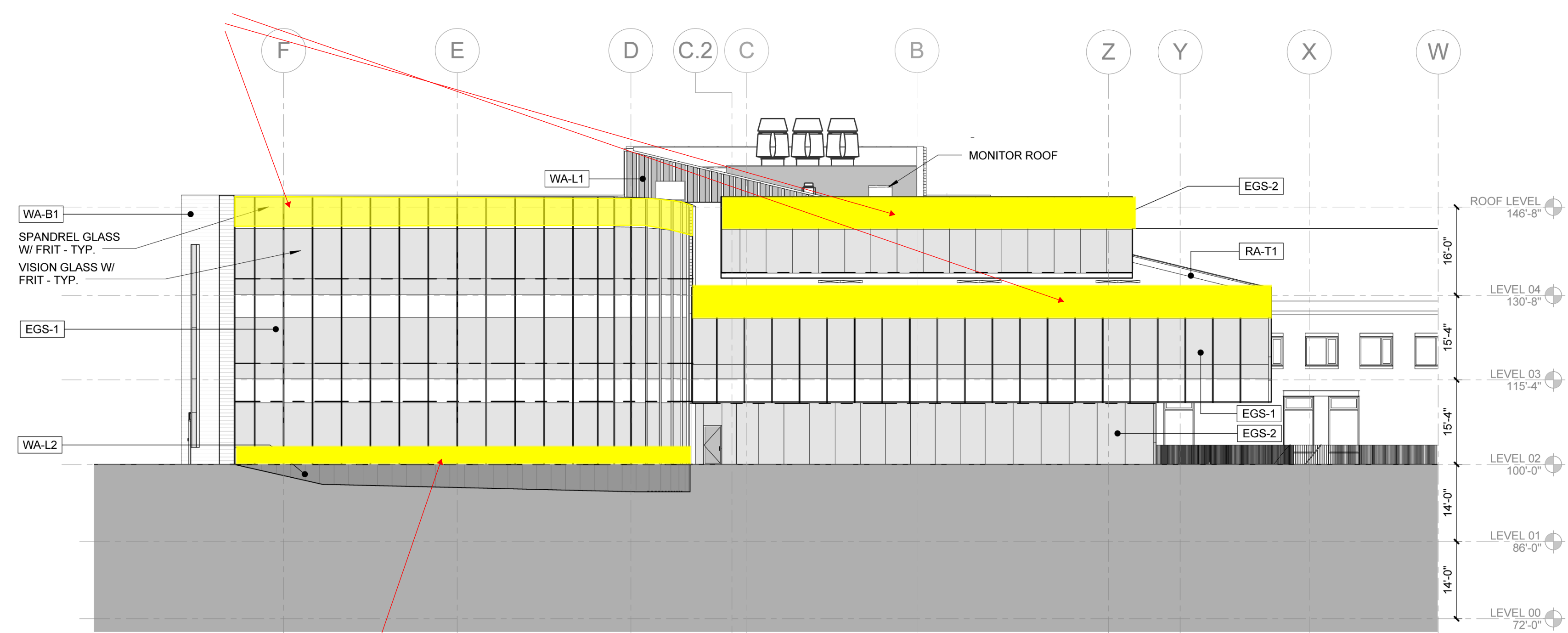
1 EXTERIOR WEST 1/16" = 1'-0"
